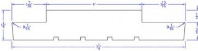
Interior Double Rabbeted Jamb
