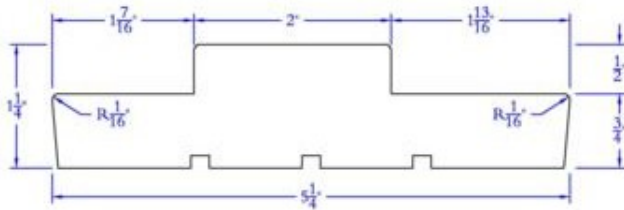
Interior Double Rabbeted Jamb
