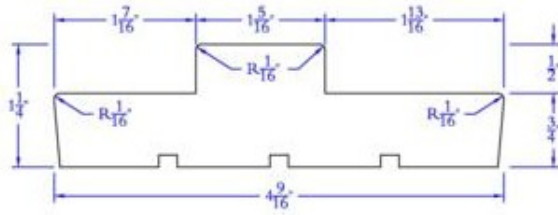
Interior Double Rabbeted Jamb
