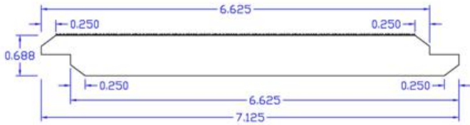
T&G and Shiplap Patterns - WP11 Texture R/S Face
